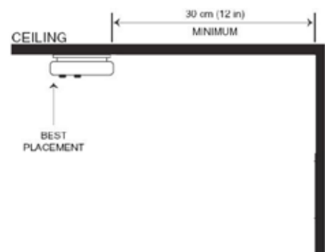
CEILING PLACEMENT
